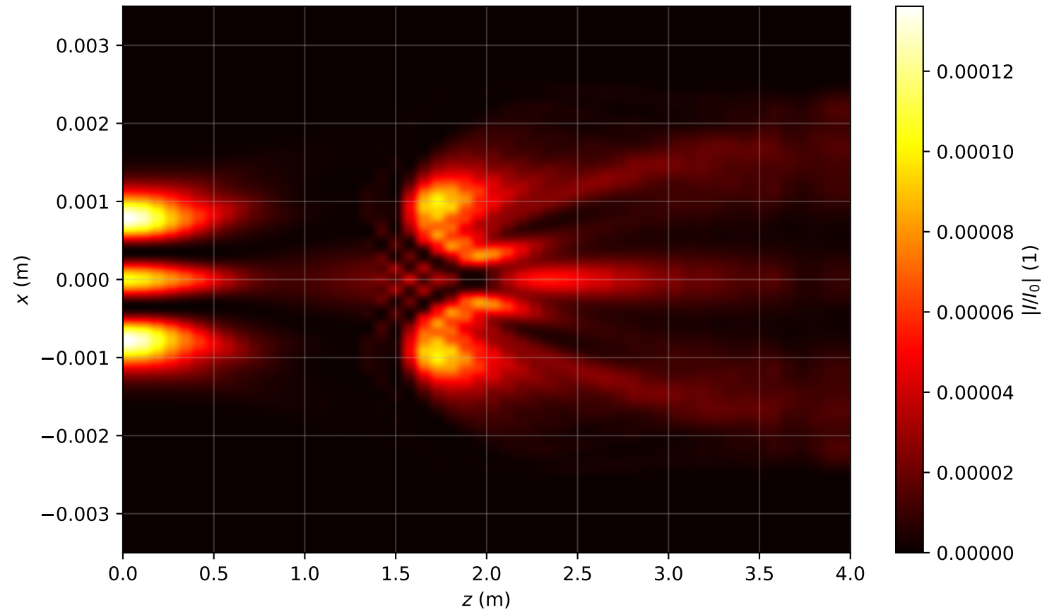
Intensity profile I(x, y = 0, z)/I_0 , P_{in}=5.0P_{cr} , artificial time
